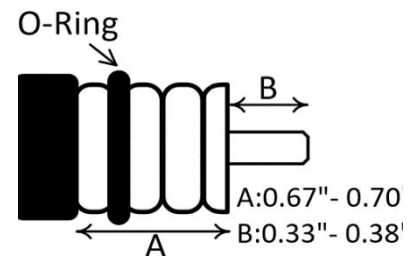
Cable Preparation Requirements
